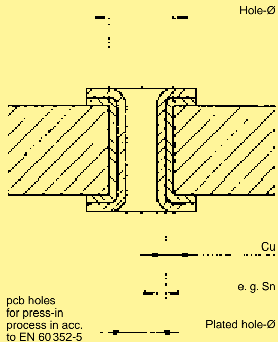
Cross section of a pcb 2.4 mm thick with various hole diameters
